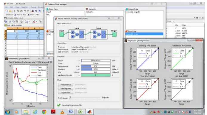
Fig.4. 3MSE Performance graph and designed network with Data Manager for Trial.
