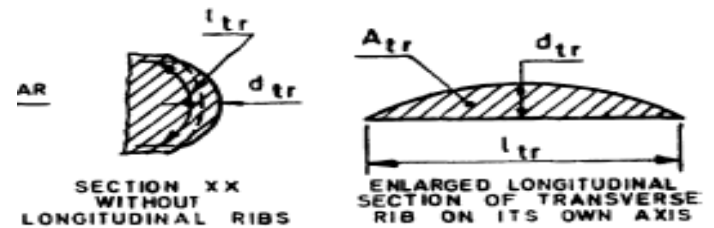
Fig.1. 1 Typical cross-section and Parameters involve of MS, CTD and TMT [3].
