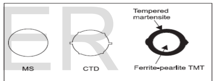
Fig.1. 1 Typical cross section of MS, CTD and TMT [3].
