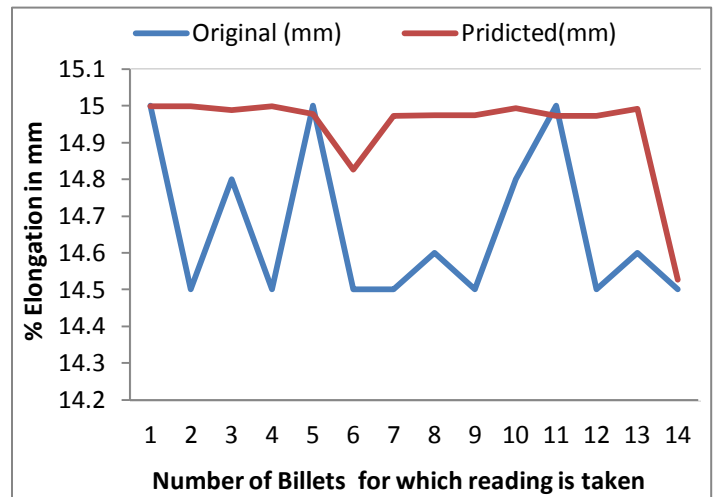
Fig.4.9 Comparison predicted and actual output of % elongation of the rolled TMT
