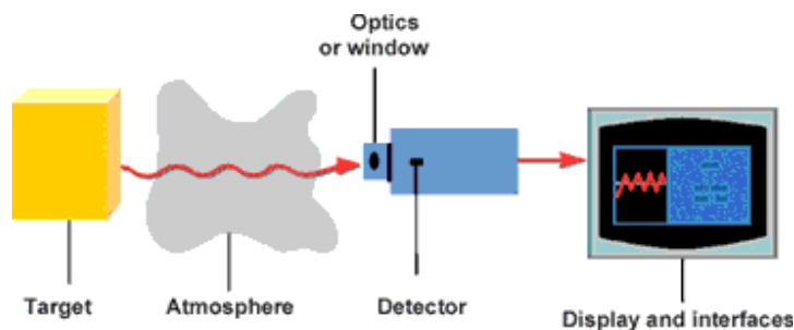
Fig.3. 1 Arrangement of pyrometer and working [16].
