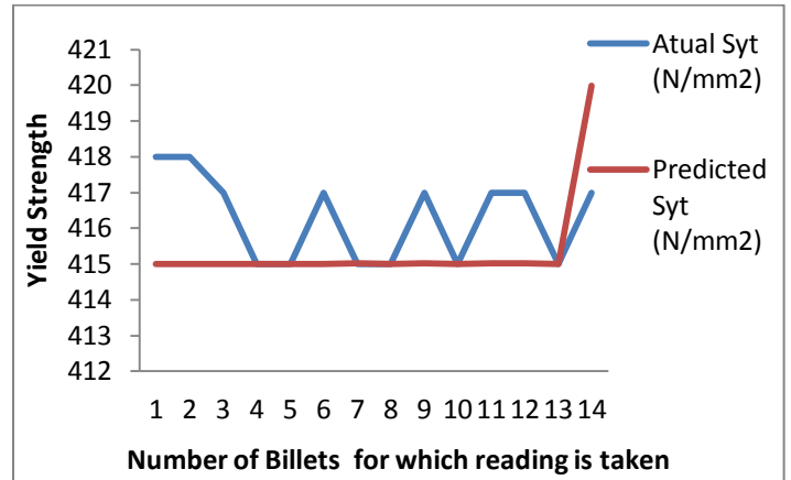
Fig.4. 7 Comparison predicted and actual output of Yield Strength of the rolled TMT.
