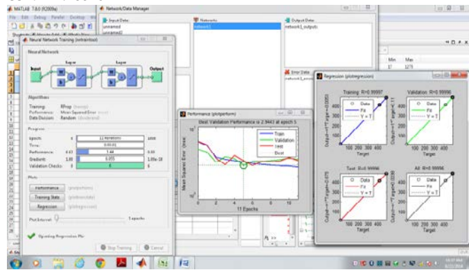
Fig.4. 1 MSE Performance graph and designed network with Data Manager for Trial No 1.
