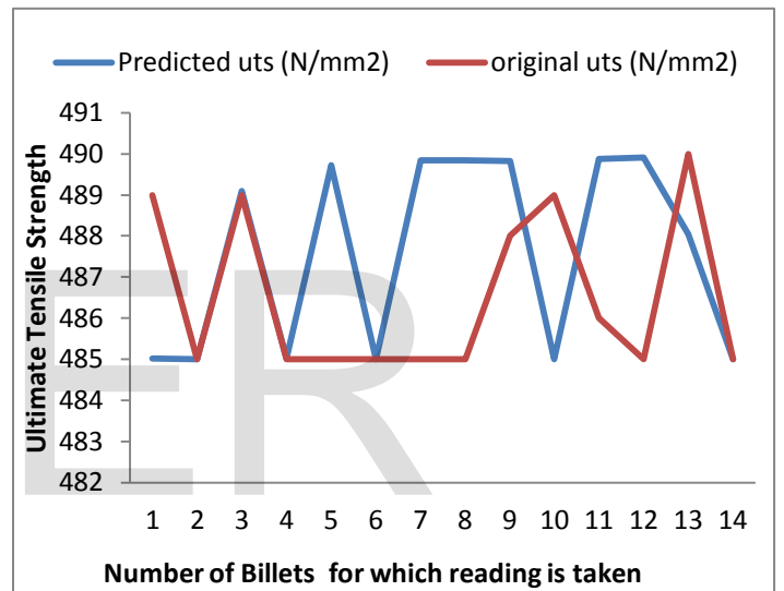
Fig.4. 8 Comparison predicted and actual output of ultimate tensile strength of the rolled TMT.
